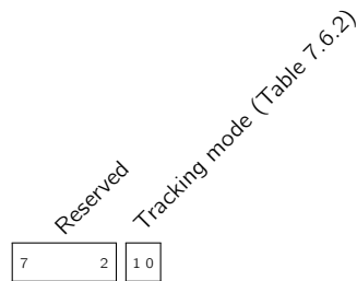
Field 7.6.1: Status of tracking channel (state)
