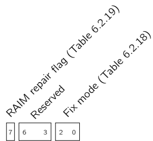
Field 6.2.7: Status flags (flags)
