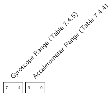
Field 7.4.2: IMU configuration (imu_conf)
