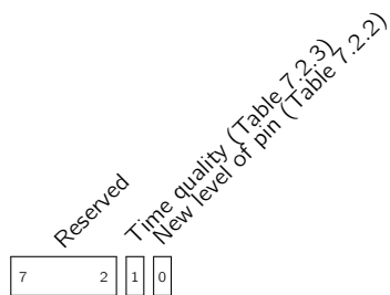
Field 7.2.1: Flags (flags)
