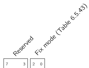
Field 6.5.17: Status flags (f1ags)
