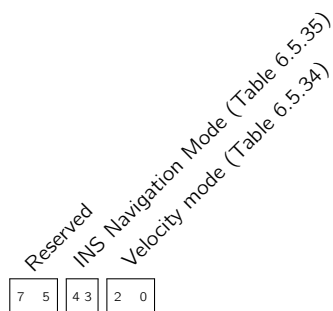
Field 6.5.13: Status flags (f1ags)
