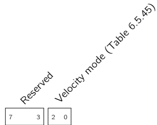
Field 6.5.18: Status flags (f1ags)
