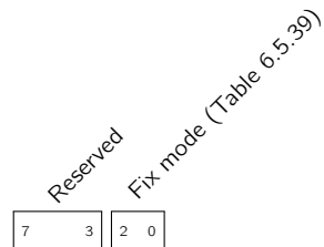
Field 6.5.15: Status flags (f1ags)
