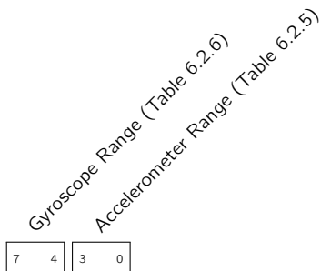
Field 6.2.3: IMU configuration (imu_conf)
