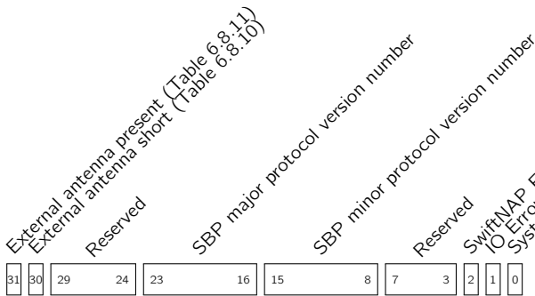
Field 6.8.4: Status flags (flags)
