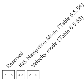
Field 6.5.22: Status flags (flags)
