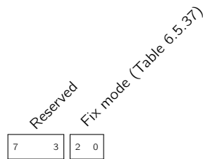
Field 6.5.14: Status flags (flags)
