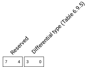
Field 6.9.3: Status flags (flags)
