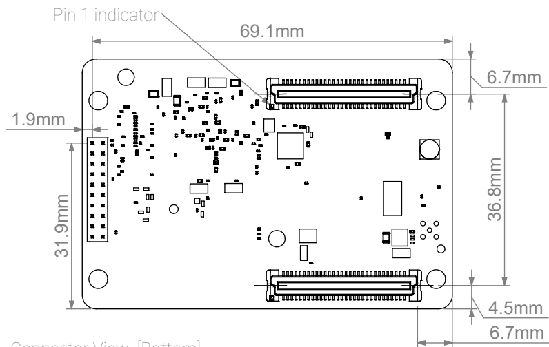
Connector View [Bottom]
