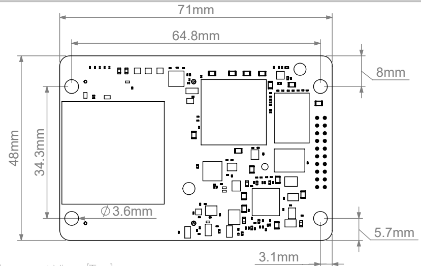
Hole Placement View [Top]
