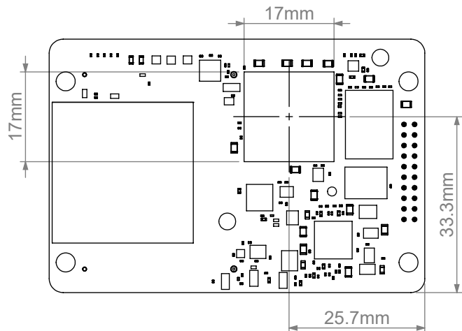
Heatsink Mating View [Top]
